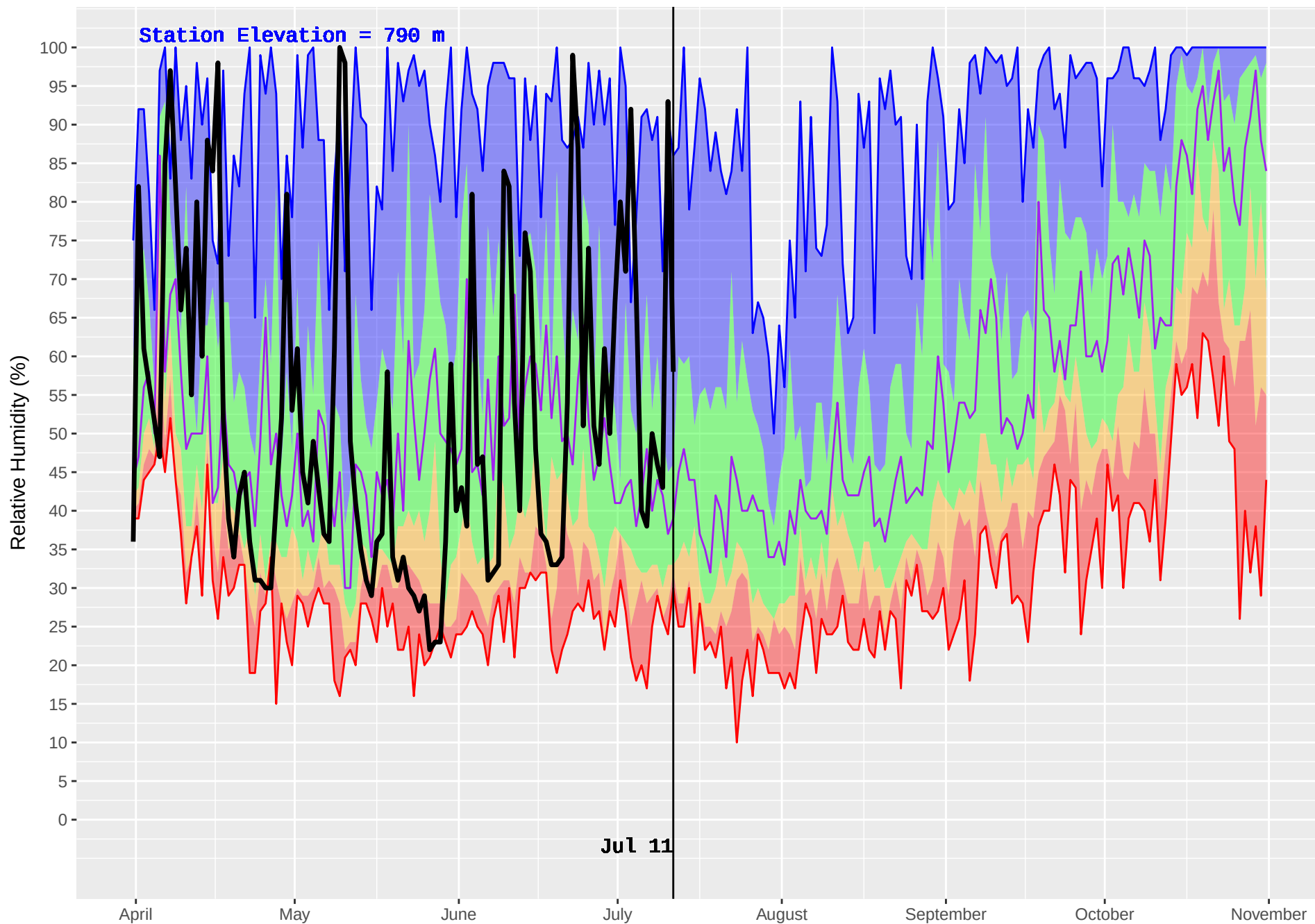
FALLS CREEK (383) : Historical (2002–2016) and Current (2018) Noon Relative Humidity
